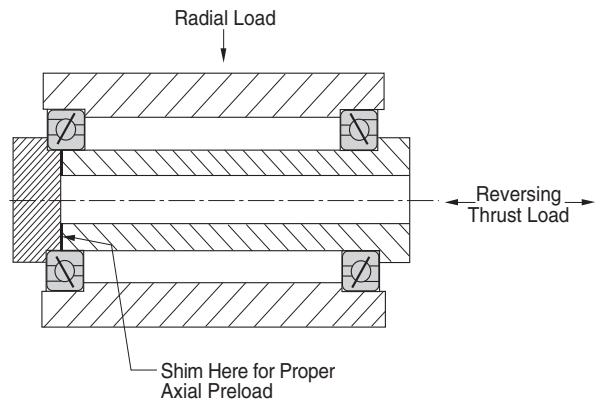
B-Type Configuration
