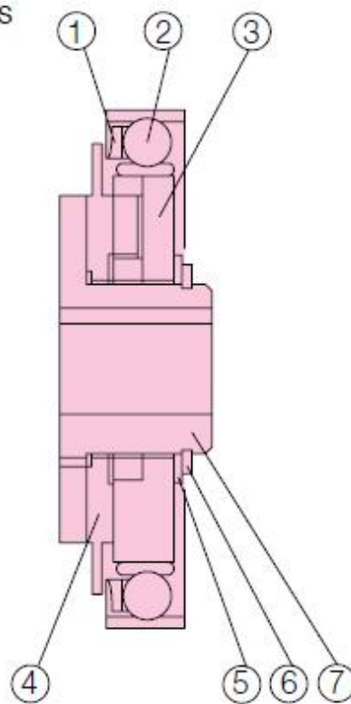
SHF-14,17,20,25,32,45,58
